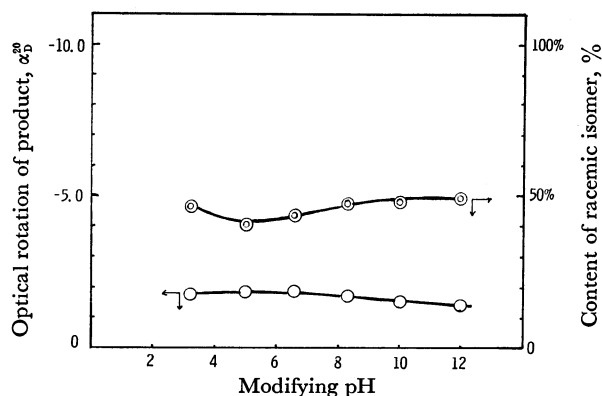
Fig. 4. Effect of modifying pH on asymmetric hydrogenation of acetylacetone using Raney nickel catalyst modified with L-glutamic acid at 0 °C and component of racemic 2,4-pentanediol.
